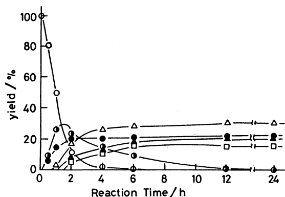
Fig. 2. Time course of the oligoadenylylates formation ImpA. Reaction conditions: ImpA, 50 mM; \text{UO}_2(\text{NO}_3)_2 , 1 mM; 20 °C; pH 7.3 ImpA, (○); \text{Im}(\text{pA})_2+\text{Im}(\text{pA})_3 , (●); (\text{pA})_2+(\text{pA})_3 , (●); (\text{pA})_4+ (\text{pA})_5 , (Δ); (\text{pA})_6-(\text{pA})_8 , (▲); (\text{pA})_9 , (□).
