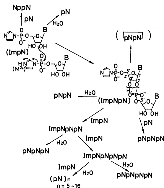
Scheme 1. Reaction scheme of the oligonucleotide formation.
